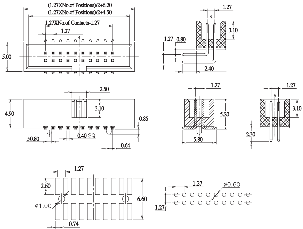
Recommended PCB Layout (PCB TOLERANCE \pm 0.05 )
